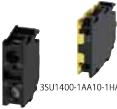
3SU1400-1AA10-1BA0
